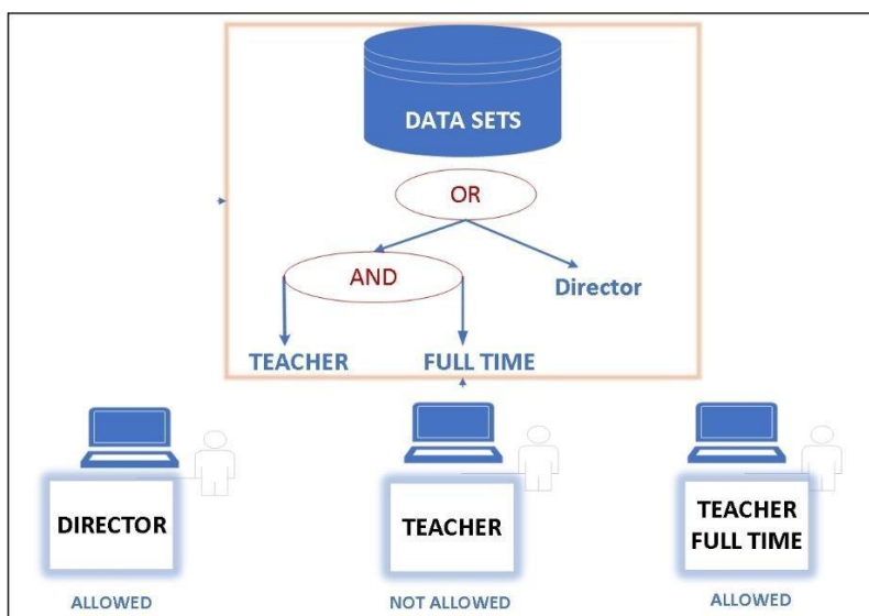
Figure 1: CP-ABE
